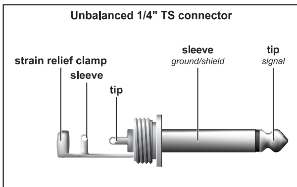
Fig. 4.3: 1/4" TS connector
